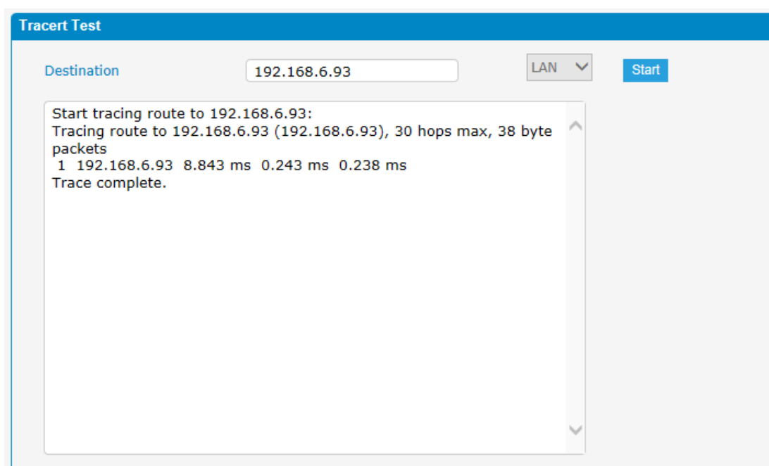
Figure 3.12.3 Tracert
